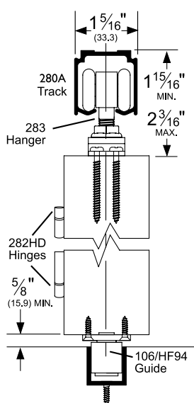
280A Overhead Mounted
