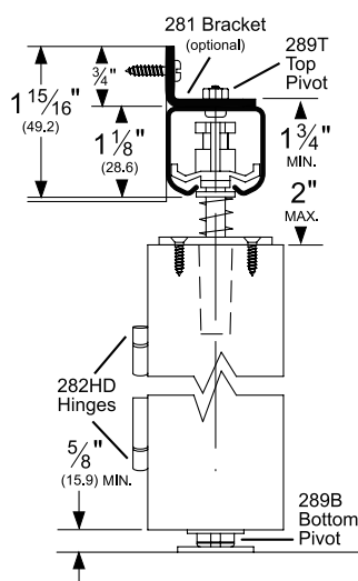
280 Side Wall Mounted
