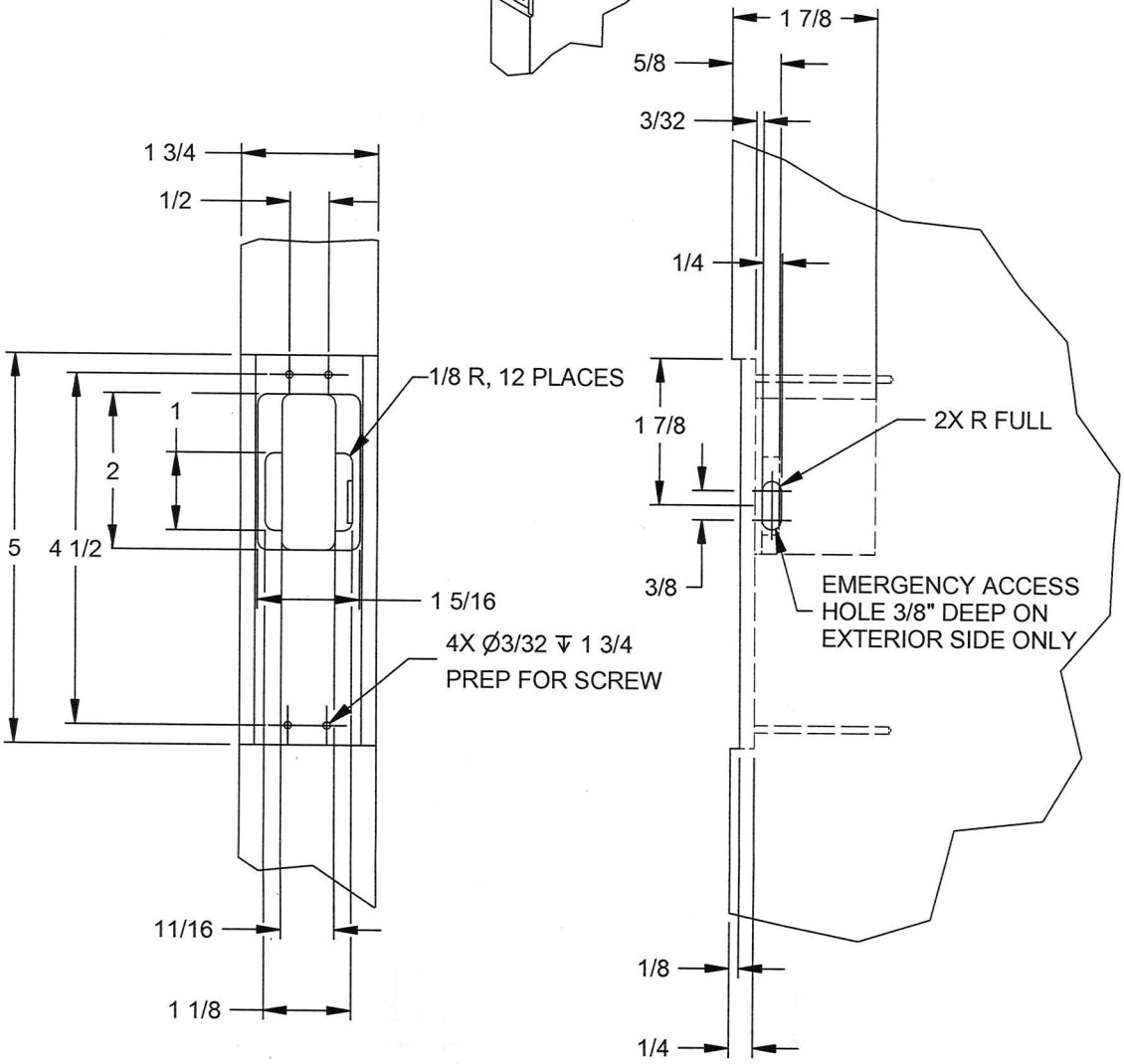
DOOR PREP FOR 1-3/4" WOOD DOOR AND WIDER CENTER PATTERN IN DOOR THICKNESS
