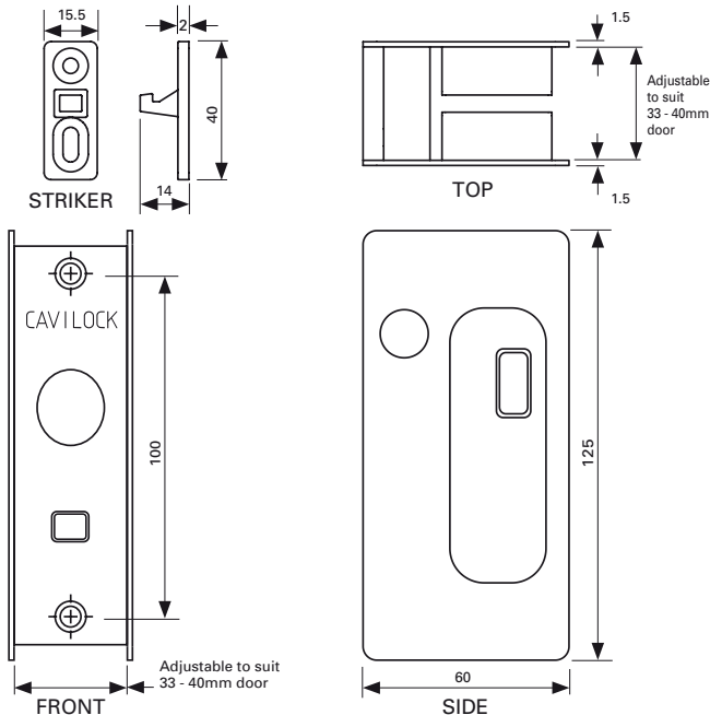
CONFIGURATION A Privacy with Right Hand Snib or Snib / Emergency (option when fitting)
