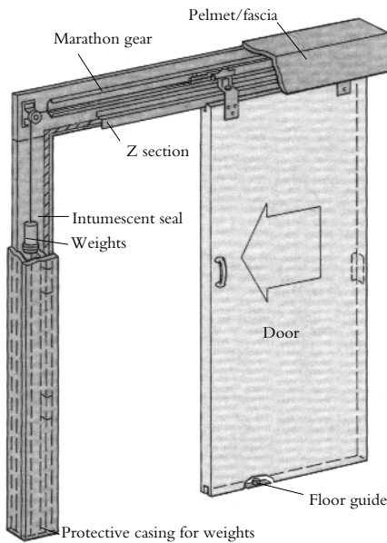
Typical installation
